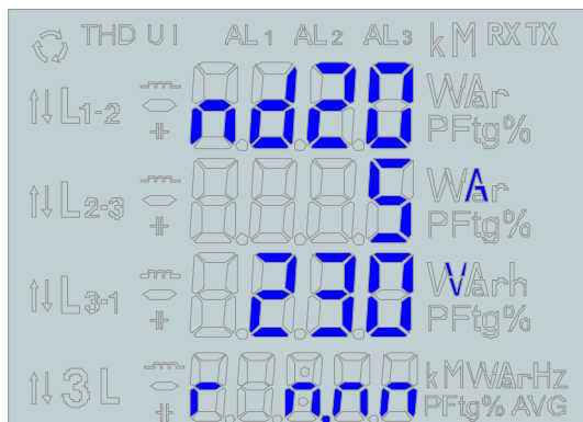
Fig. 6. Message after starting the meter
