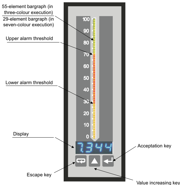
Fig. 4 Description of the NA5 frontal plate.
