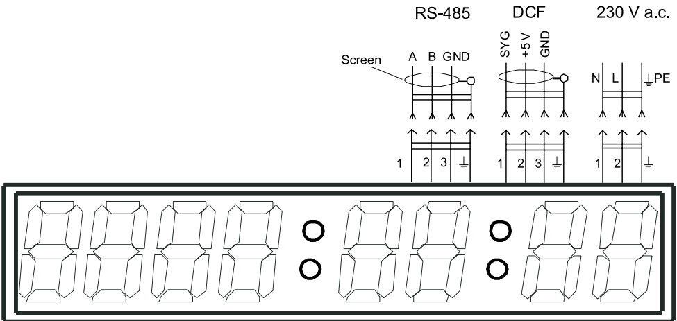
Fig. 3. Electrical connections
