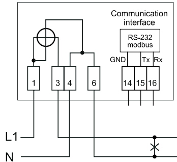
Watt-hour meter with an RS-232 communication interface and Modbus protocol
