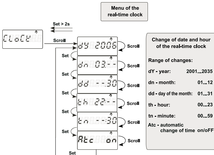
Fig. 12c Algorithm of the watt-hour meter work - menu of the real-time clock
