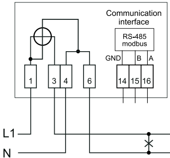
Watt-hour meter with an RS-485 communication interface and Modbus protocol
