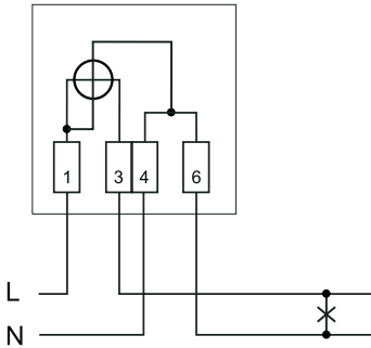
Single-tariff watt-hour meter for direct connection
