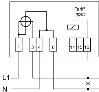
Two-tariff watt-hour meter with an external clock
