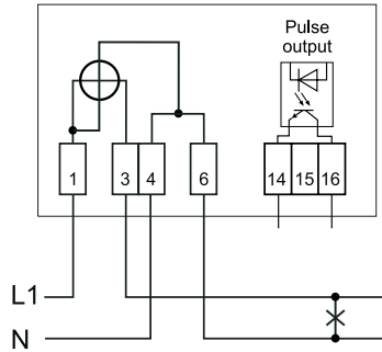
Watt-hour meter with pulse output
