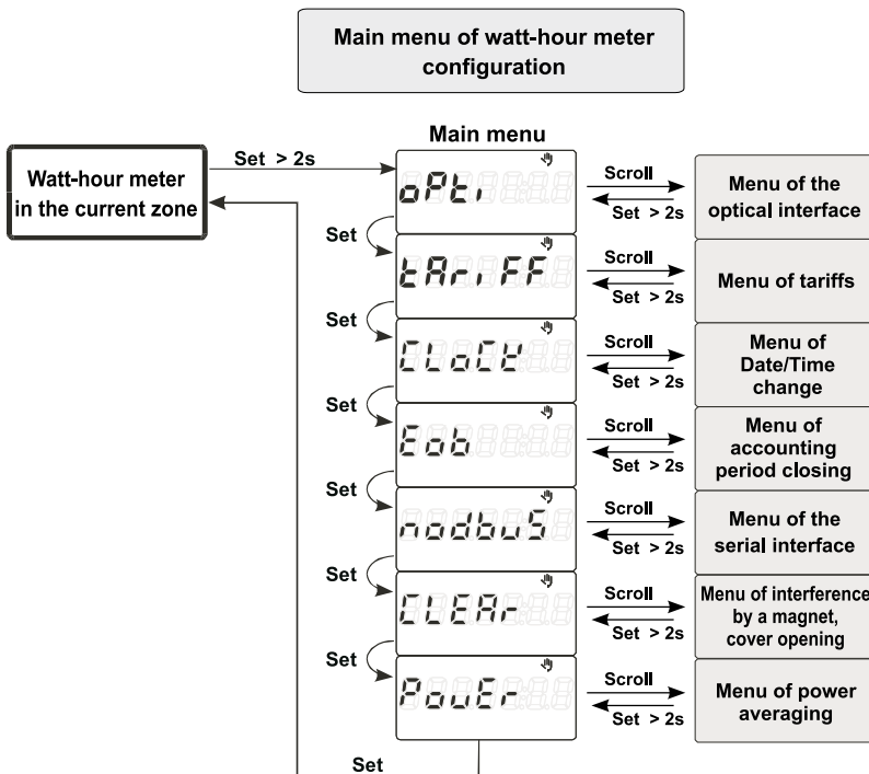
Fig. 12a Watt-hour work algorithm - Main menu
