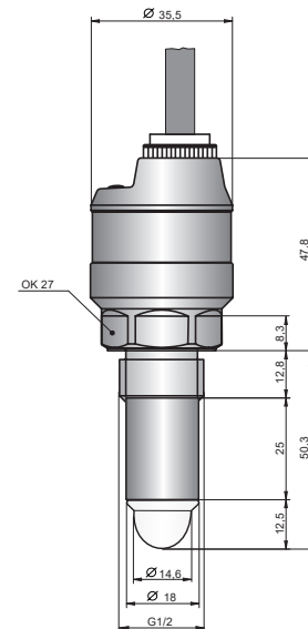
RFLS-35_-11-G1/2
