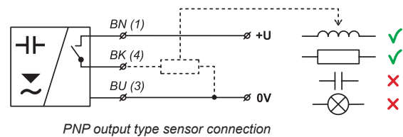
PNP output type sensor connection
